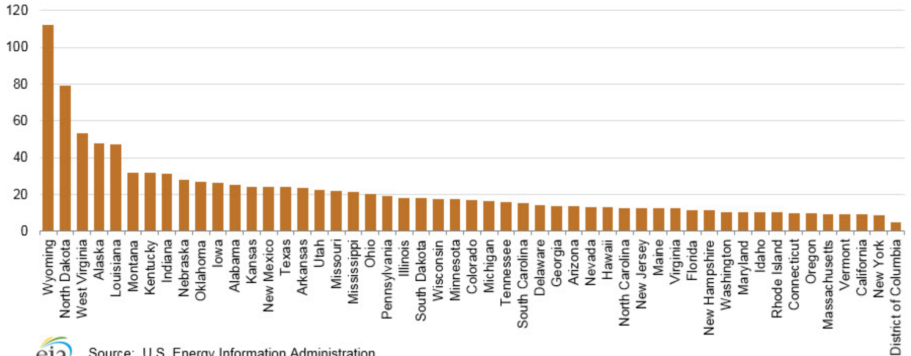
Figure 2. Per-capita energy-related carbon dioxide emissions by state, 2014
